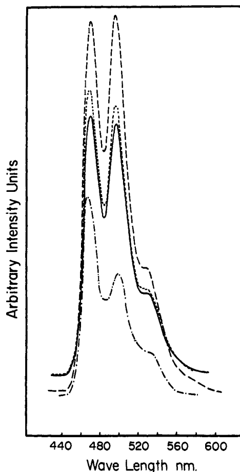
Figure 1. The chemiluminescence emission spectrum of 10^{-4} M 1 in dimethyl sulfoxide with sodium hydroxide (—), fluorescence emission spectrum of the spent reaction mixture (----), fluorescence emission spectrum of acridone ( 5 ) (· · · · ·), and 9-acridinecarboxylic acid ( 9 ) (- · - · -); the latter two are 10^{-4} M in dimethyl sulfoxide with sodium hydroxide present as the base.
