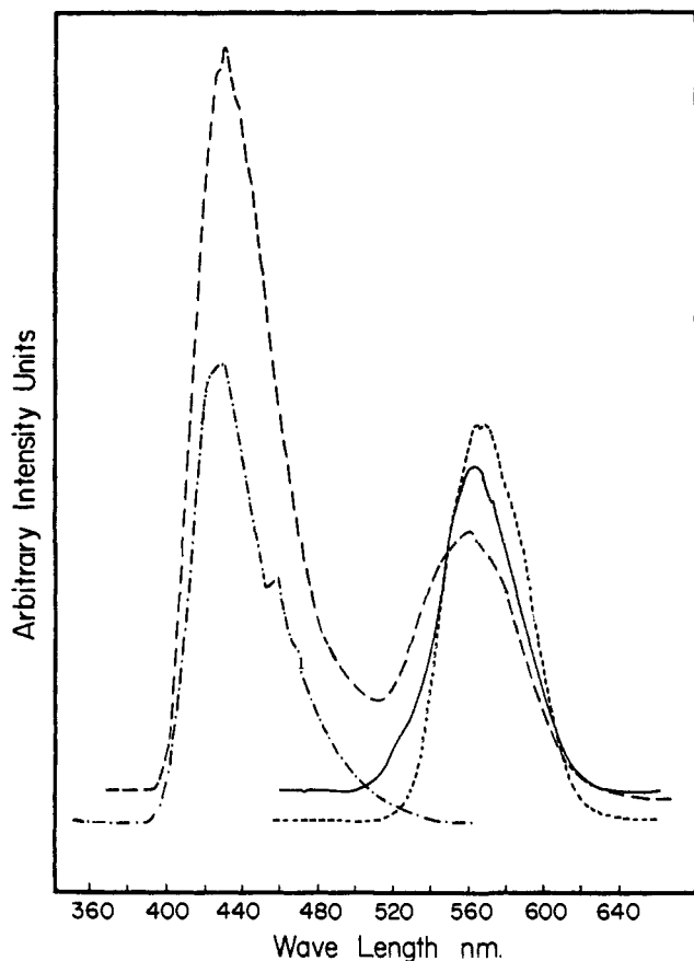
Figure 3. The chemiluminescence emission spectrum of 10^{-4} M 11 , in dimethoxyethane with the radical anion of naphthalene 10^{-2} M in dimethoxyethane (—), fluorescence emission spectrum of the spent reaction mixture (---), fluorescence emission spectrum of 9-anthracenecarboxylic acid ( 13 ) (-·-·-·-), and anthrone ( 12 ) (-----); the latter two are 10^{-4} M in dimethoxyethane with the radical anion of naphthalene in dimethoxyethane 10^{-2} M, or with potassium tert -butoxide in dimethoxyethane as bases.
